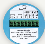
4-Channel Base
